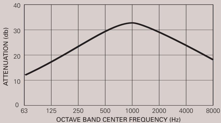
REPRESENTATIVE ATTENUATION CURVE FOR "TBU" SERIES SILENCERS
